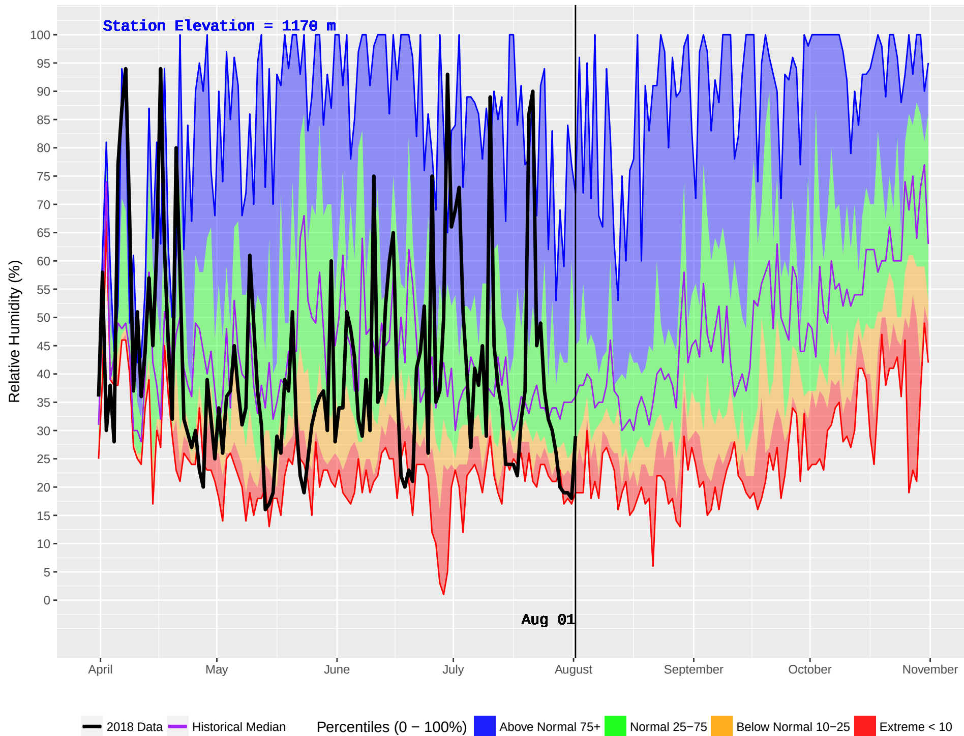
YOUNG LAKE (235) : Historical (2001–2016) and Current (2018) Daily Relative Humidity
