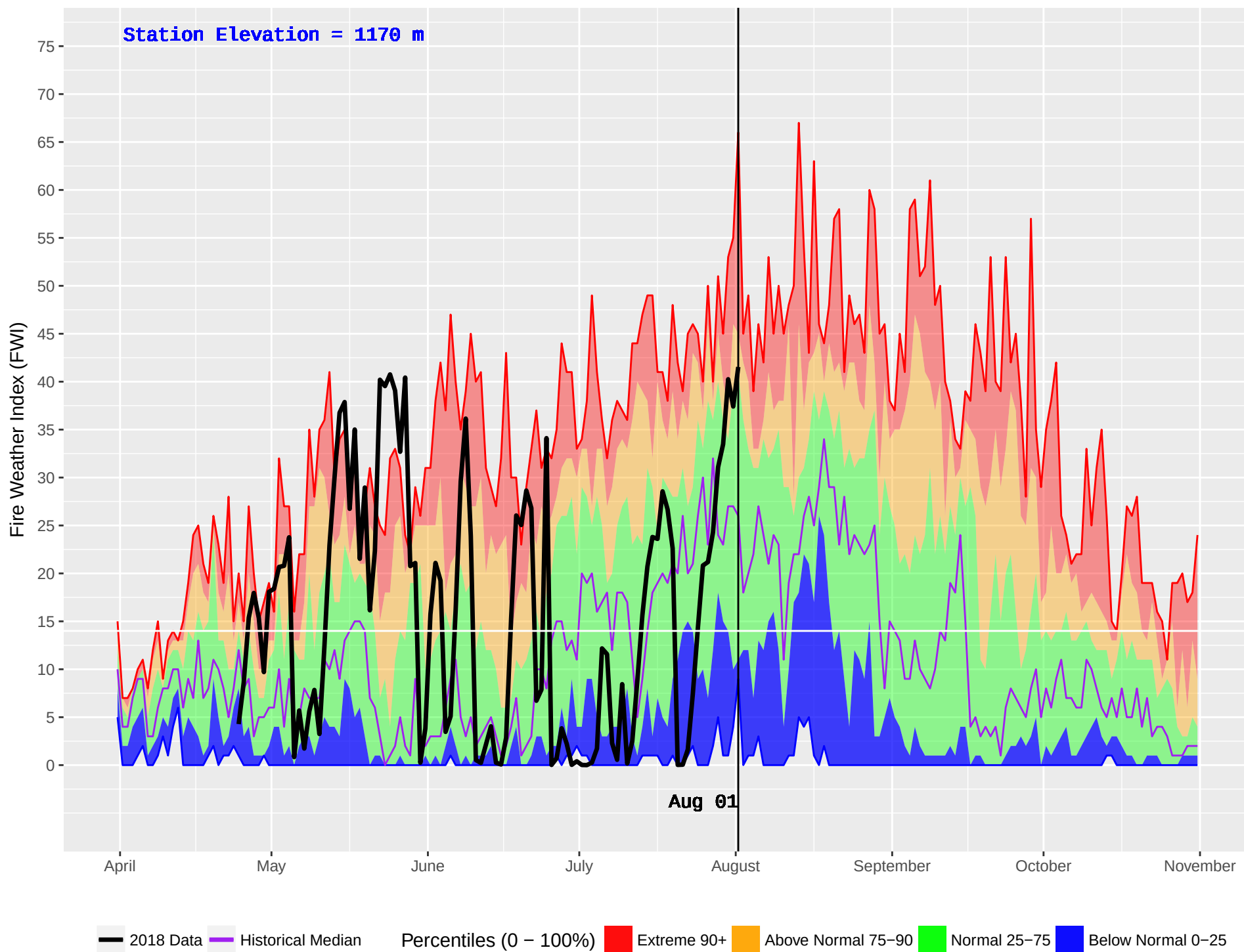
YOUNG LAKE (235) : Historical (2001–2016) and Current (2018) Daily Fire Weather Index (FWI)
