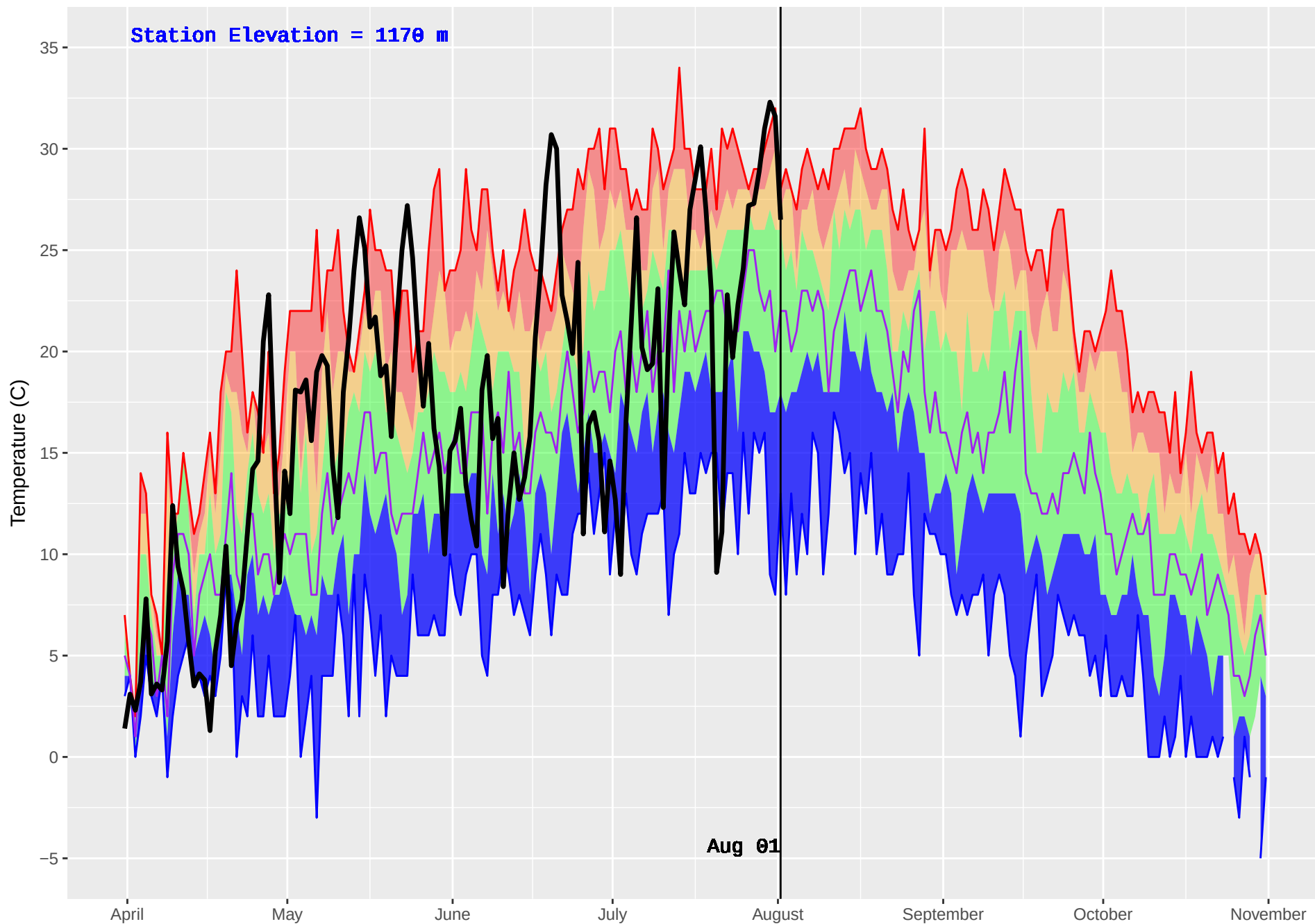
YOUNG LAKE (235) : Historical (2001–2016) and Current (2018) Daily Temperature
