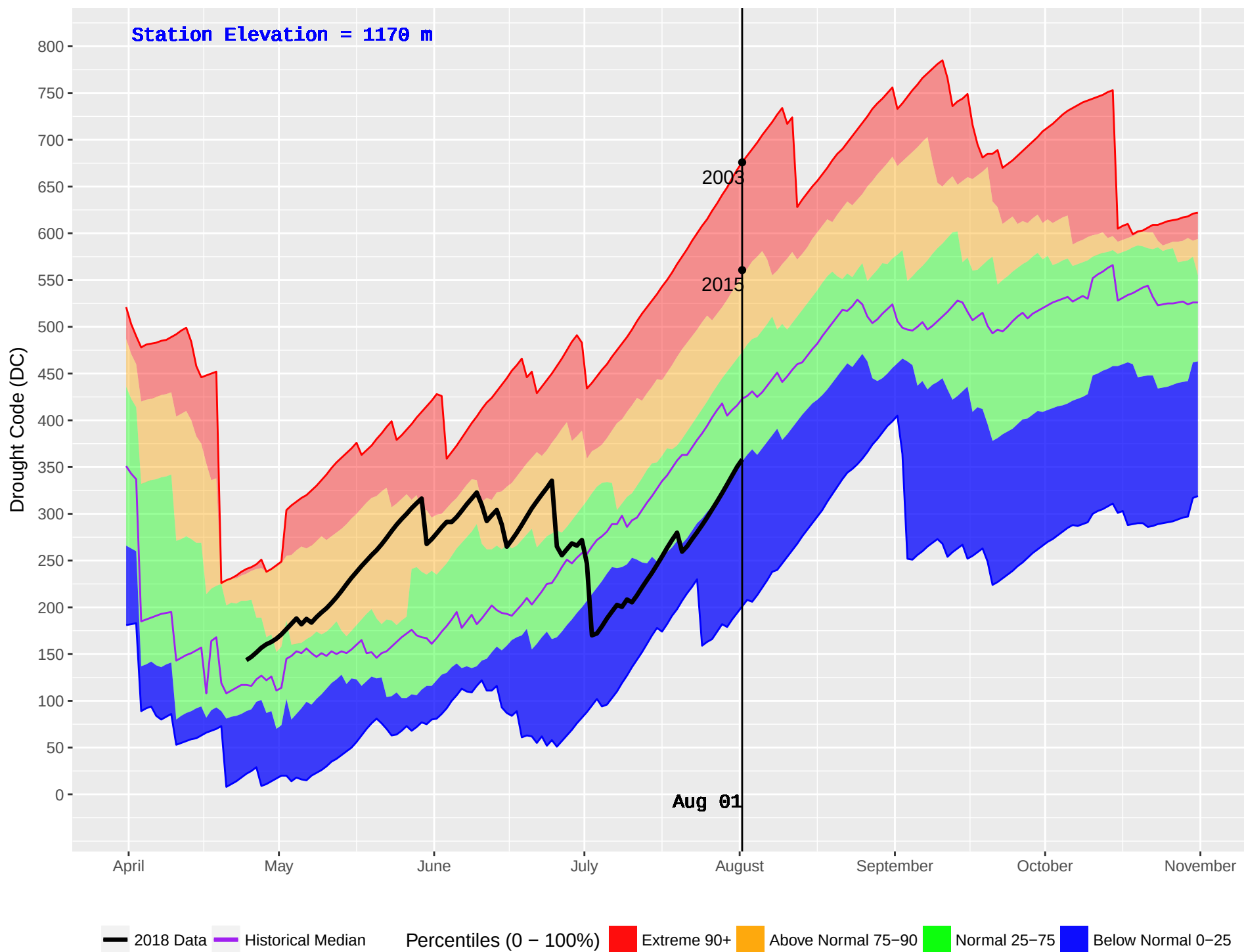
YOUNG LAKE (235) : Historical (2001–2016) and Current (2018) Daily Drought Code (DC)
