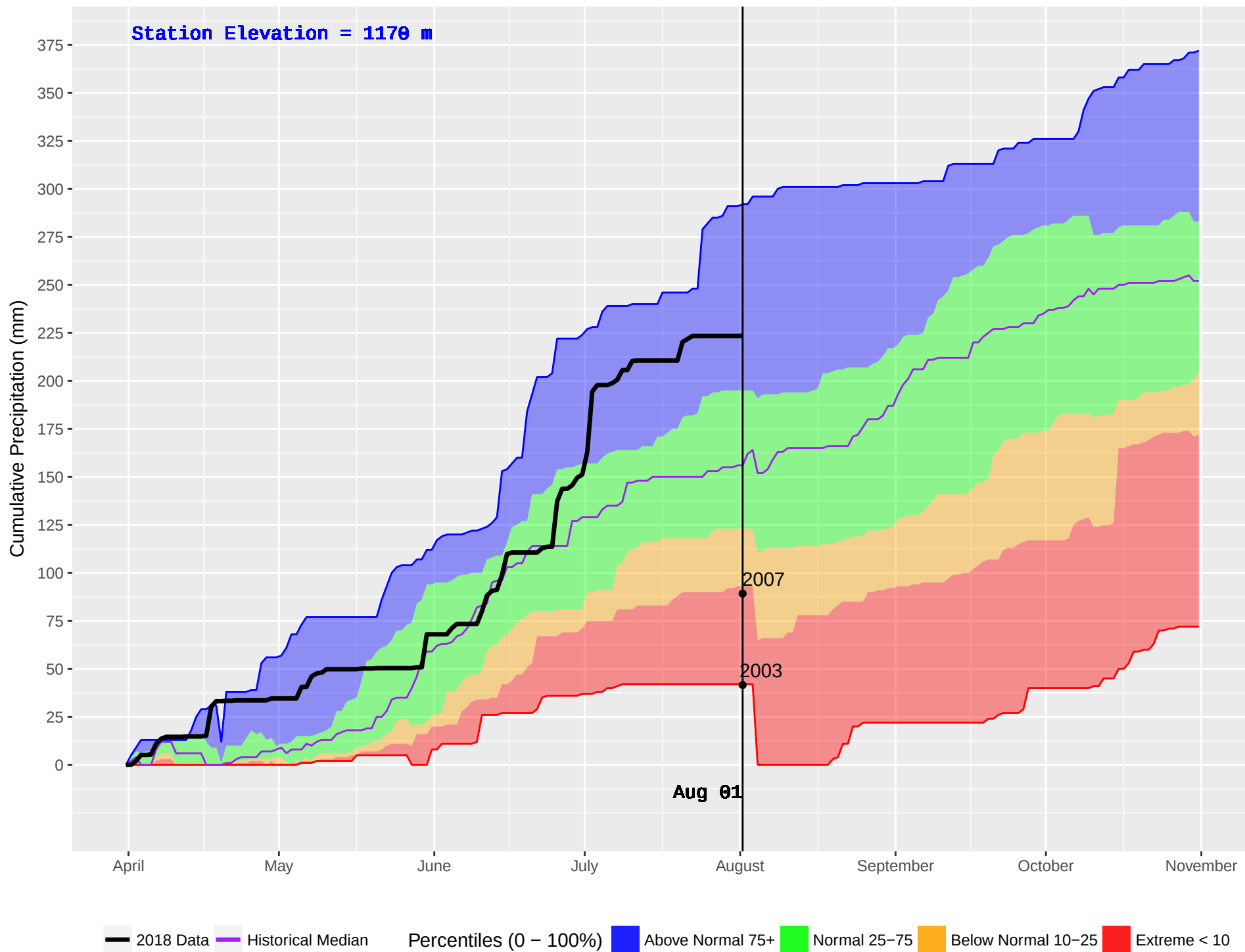
YOUNG LAKE (235) : Historical (2001–2016) and Current (2018) Daily Cumulative Precipitation
