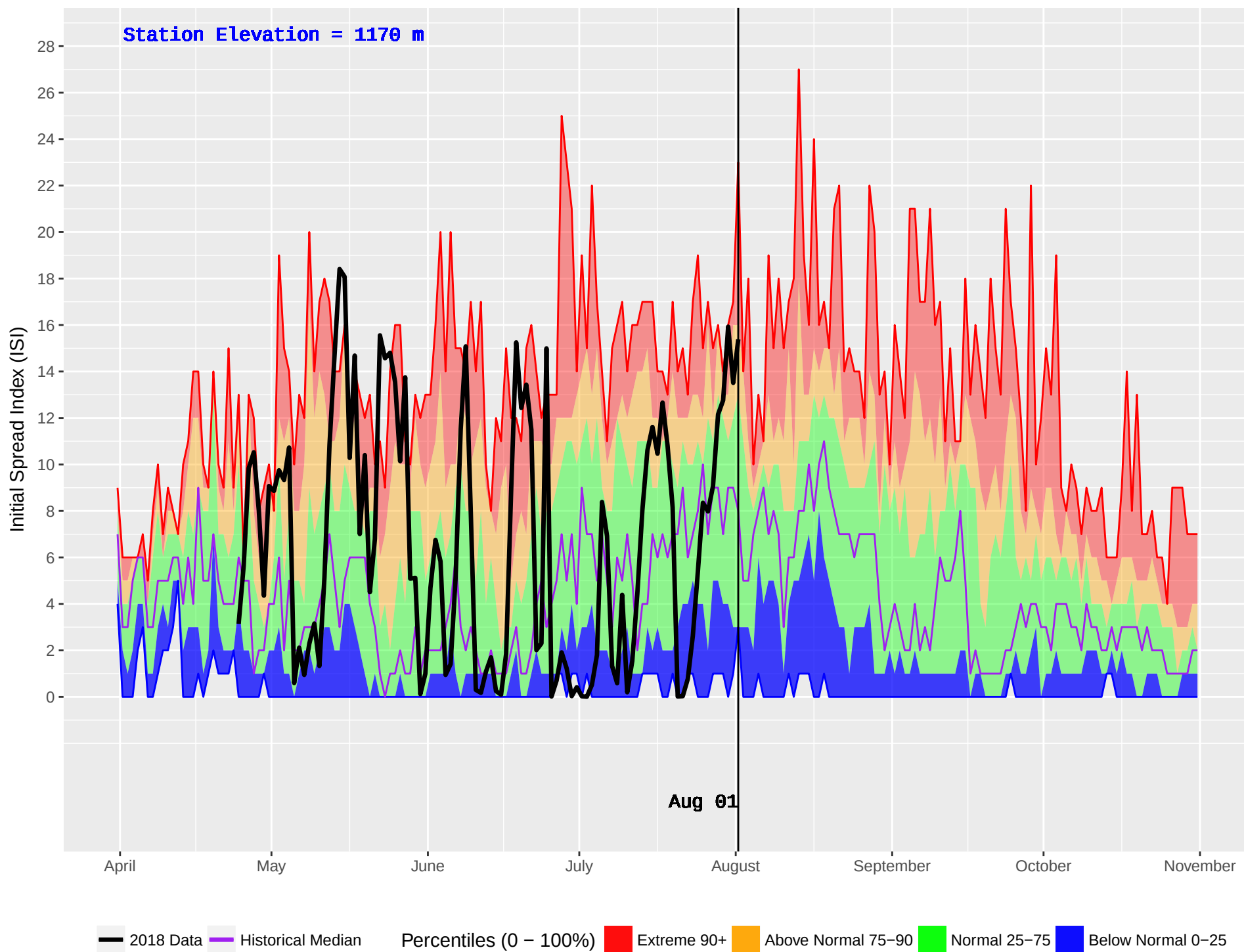
YOUNG LAKE (235) : Historical (2001–2016) and Current (2018) Daily Initial Spread Index (ISI)
